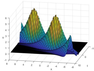
(n) u-x-t with c_2 = 2
