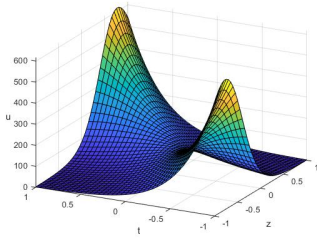
(c) u-z-t with c_3 = 1
