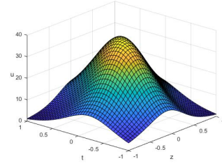
(e) u-z-t with c_3 = -2
