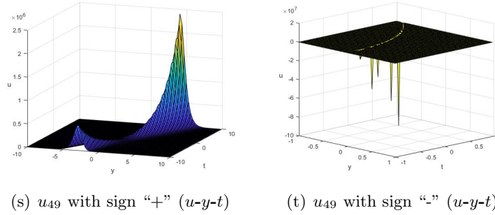
Fig.7 u_{49} as a_2 = a_3 = a_4 = 1, k_3 = 1, c_3 = 1, l_3 = -1, l_2 = l_4 = -\frac{1}{2}, x = z = 0 .
