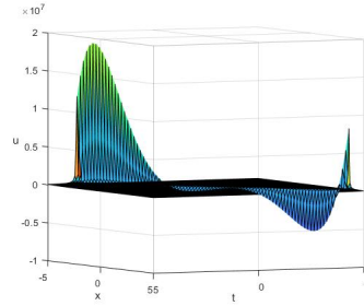
(j) u_{14} with c_4 = 1 ( u-x-t )
