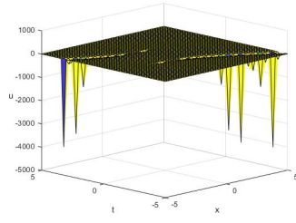
(g) u-x-t with sign “-”
