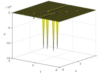
(h) u-x-t with sign “+”
