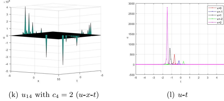
Fig.4 periodic two solitary solution as
