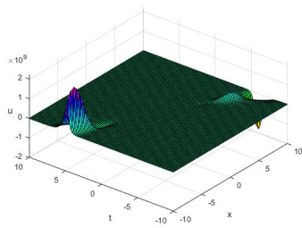
(i) u_{12} with c_4 = 2 ( u-x-t )
