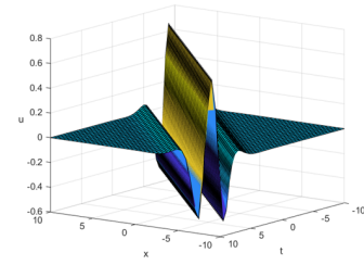
(o) u-x-t with c_2 = 1
