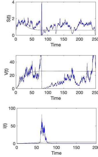
Figure 2. The blue lines show the paths of S(t), V(t), I(t) with jump noise under the noise intensities (\sigma_1^2, \sigma_2^2, \sigma_3^2) = (0.04, 0.16, 0.8) , (\eta_1, \eta_2, \eta_3) = (0.1, 0.1, 0.8) . The black ones are the paths of deterministic SVI model.
