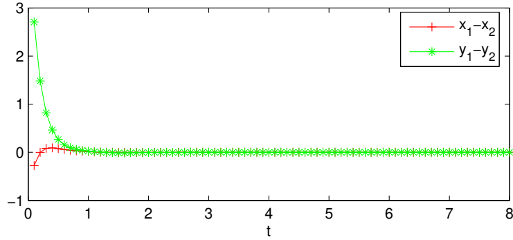
Fig. 1 The differences x_1 - x_2 and y_1 - y_2 to (27) and (28) computed by 2-degree DG method
