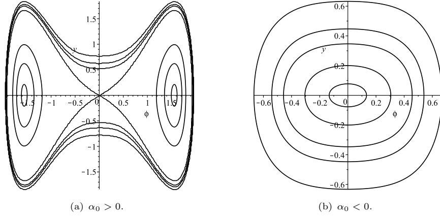
Figure 2. Phase portraits of system (5) when F(\psi) has one positive zero or has no zero.
