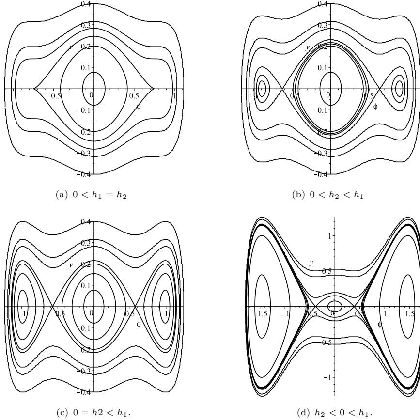
Figure 1. The bifurcations of phase portraits of system (5) when \alpha_0 < 0, \alpha_2 > 0, \Delta > 0 .
