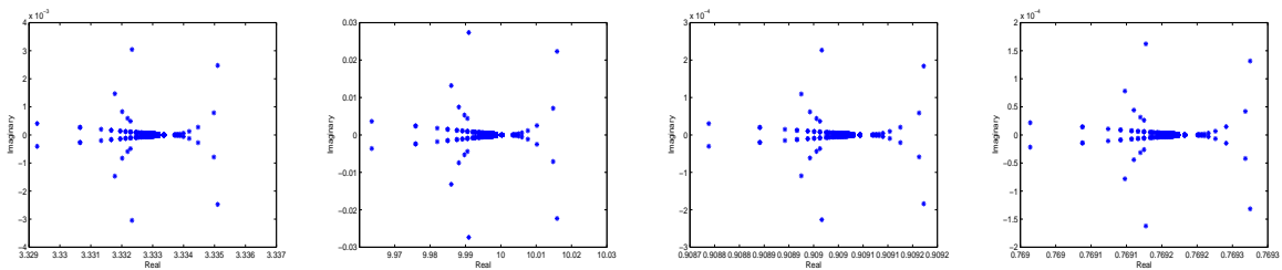
Figure 2: The eigenvalue distribution for the parameter shift-splitting preconditioned matrix \mathcal{T}_{PSS}^{-1} \mathcal{A} when \alpha = \beta = 0.001, \xi = 0.5 (the first), \alpha = \beta = 0.001, \xi = 0.3 (the second), \alpha = \beta = 0.001, \xi = 0.1 (the third) and \alpha = \beta = 0.001, \xi = 1.3 (the fourth), respectively. Here, l = 16 .
