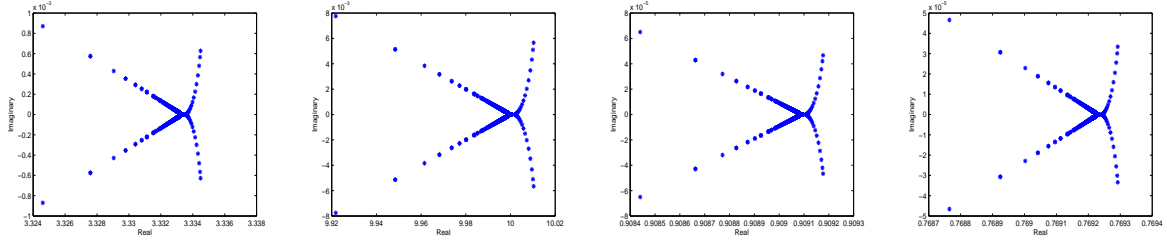
Figure 4: The eigenvalue distribution for the parameter shift-splitting preconditioned matrix \mathcal{T}_{PSS}^{-1}\mathcal{A} when \alpha = \beta = 0.001, \xi = 0.5 (the first), \alpha = \beta = 0.001, \xi = 0.3 (the second), \alpha = \beta = 0.001, \xi = 0.1 (the third) and \alpha = \beta = 0.001, \xi = 1.3 (the fourth), respectively. Here, l = 24 .
