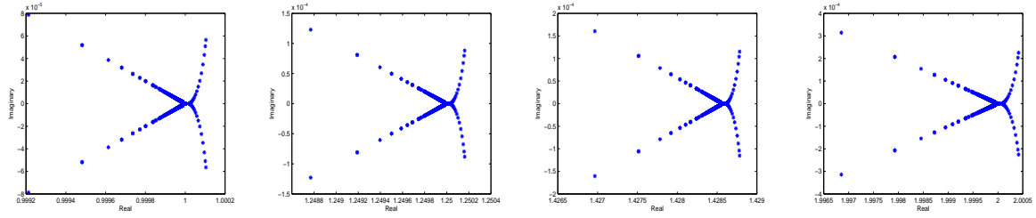
Figure 3: The eigenvalue distribution for the generalized shift-splitting preconditioned matrix \mathcal{T}_{GSS}^{-1}\mathcal{A} when \alpha = \beta = 0.001 (the first), the parameter shift-splitting preconditioned matrix \mathcal{T}_{PSS}^{-1}\mathcal{A} when \alpha = \beta = 0.001, \xi = 0.8 (the second), \alpha = \beta = 0.001, \xi = 0.7 (the third) and \alpha = \beta = 0.001, \xi = 0.5 (the fourth), respectively. Here, l = 24 .
