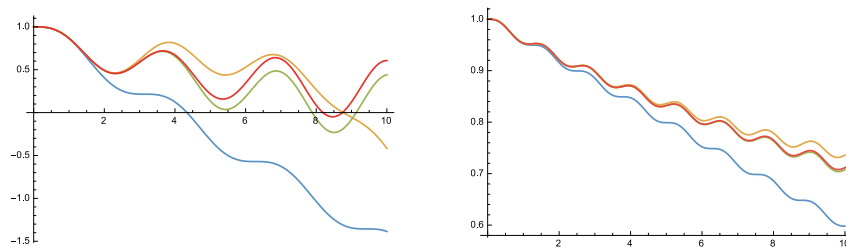
Figure 2. These graphs show the exact solution y(x) (red) for x \in [0, 10] , and the approximations y_1(x) (blue), y_2(x) (gold) and y_3(x) (green) for \Lambda = 5 (left picture) and \Lambda = 10 (right picture).
