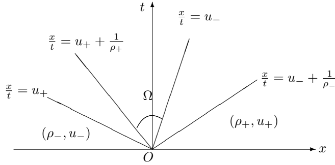
Figure 2. (t, x) -plane.
